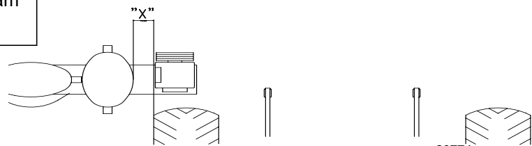
TRACTOR WHEEL ARRANGEMENT TO MOWER CUTTER BLADE. "X" DIMENSION SHOULD BE 4" OR MORE.
